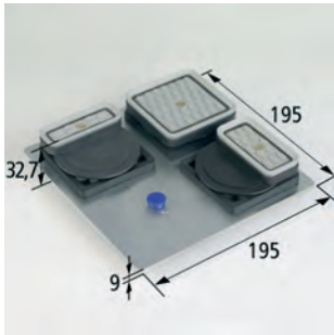
Adapter-Plate ISAP-S1 195x195x9
